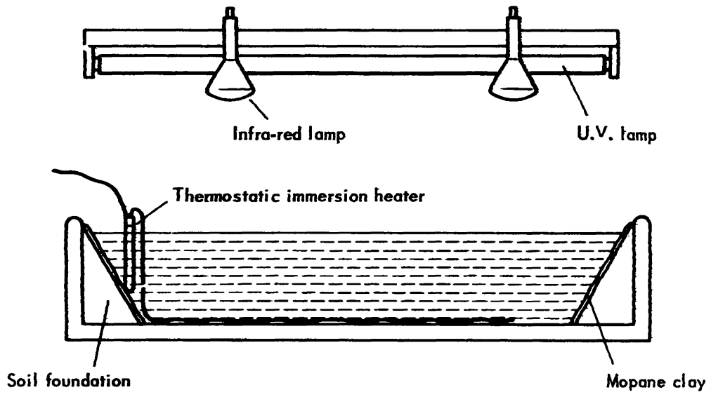
FIG. 3 ARRANGEMENT OF SINK No. S 4
