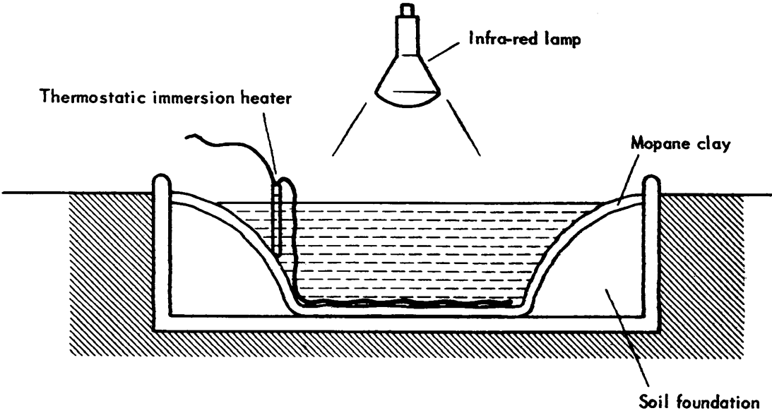
FIG. 2 ARRANGEMENT OF SINK No. S 1
